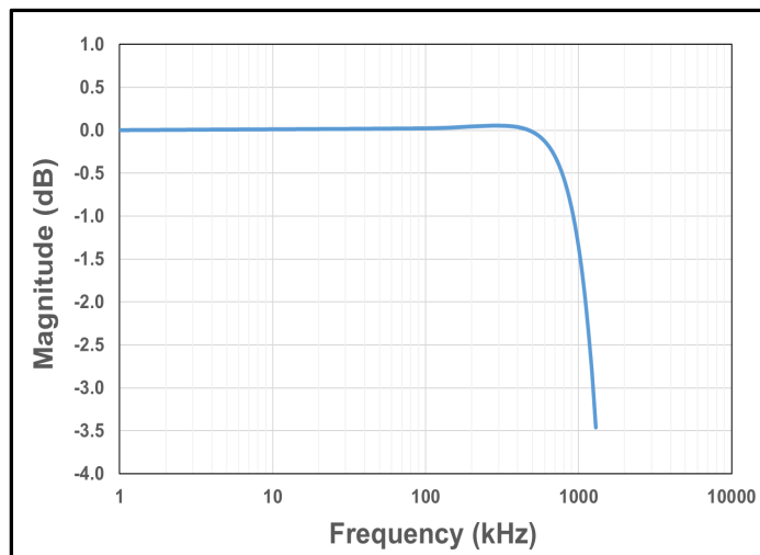
Figure 10. CT450 Bandwidth
