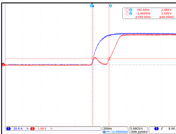
Figure 13. CT450 Propagation Delay; B_{OP} = 12\text{ mT} and C_L = 220\text{ pF} (Blue = I_{CCC} , Red = V_{OUT} )
